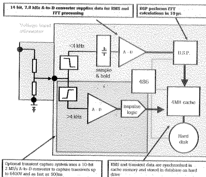
Power Recorder Architecture
